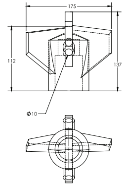
T-52 175mm Stepped Claybit
